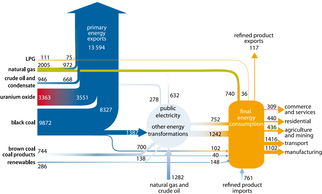
Figure E I Australian energy flows in petajoules, 2009–10
