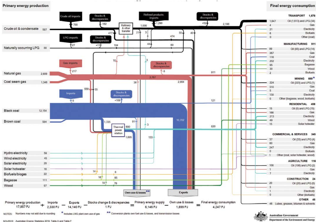
Figure E I Australian energy flows in petajoules, 2016–17
