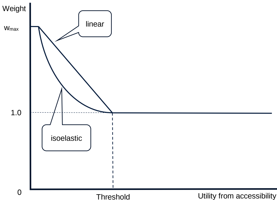
Figure 6.3 Sufficientarian – prioritarian weighting functions
