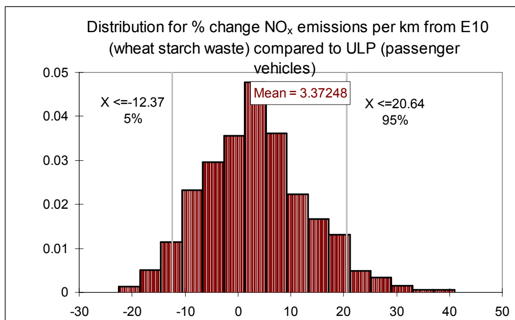
Figure A101. Distribution of percentage change in NO x emissions from E10 (wheat starch waste) compared to ULP (passenger vehicle)
