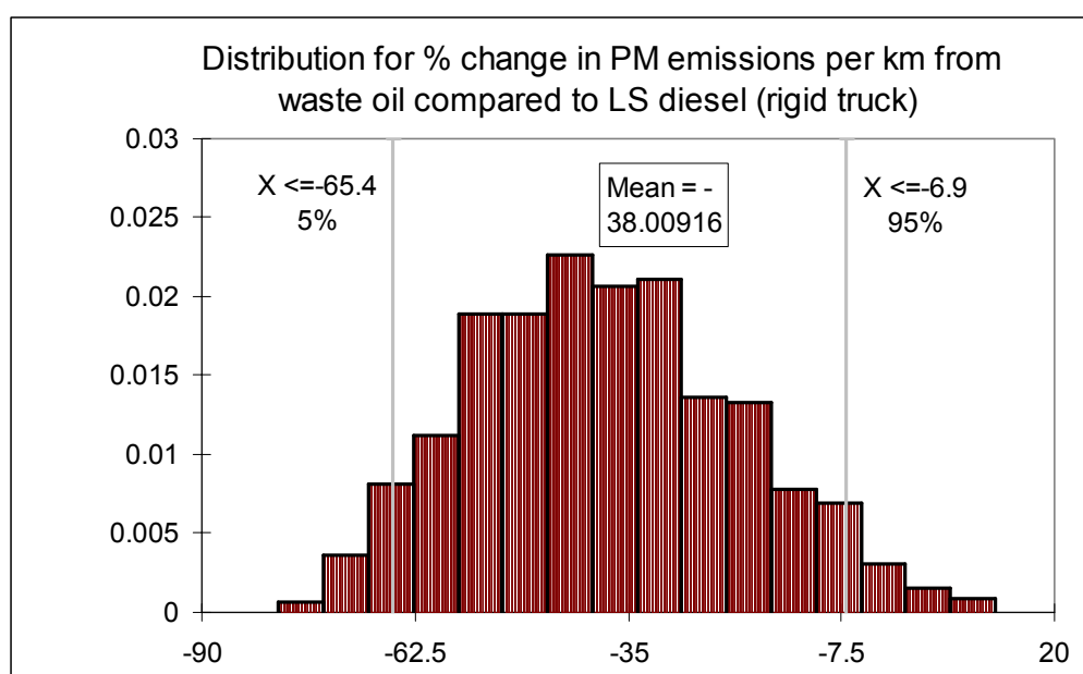
Figure A123. Distribution of percentage change in PM emissions per km from BD100 (waste oil) compared to LSD (rigid truck)
