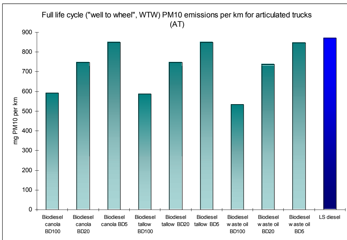
Figure A38. Fuel life cycle PM emissions from biodiesel BD100, BD20, and BD5, compared to LSD (AT)
