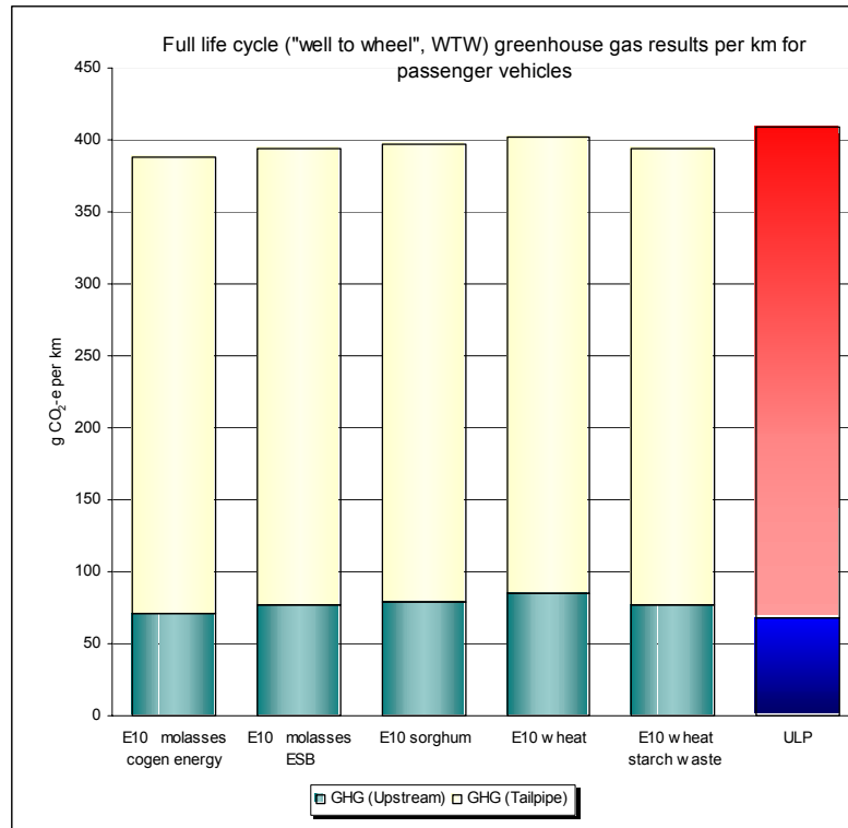
Figure A13. Fuel life cycle greenhouse gases from E10 and ULP separate for upstream and tailpipe (passenger car) 14
