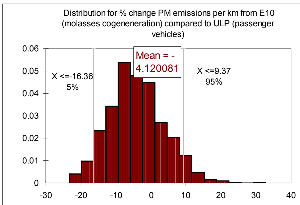
Figure A103. Distribution of percentage change in PM emissions from E10 (molasses cogeneneration) compared to ULP (passenger vehicle)
