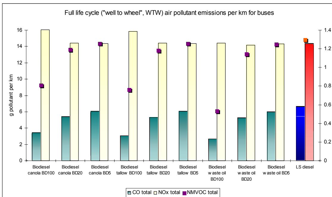
Figure A33. Fuel life cycle CO, NO x , and NMVOC emissions from biodiesel BD100, BD20, and BD5, compared to LSD (buses)
