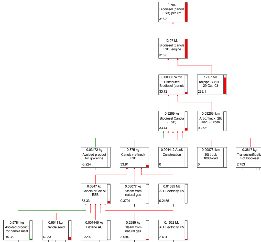
Figure A84. Biodiesel (BD100 - canola) emissions in mg PM per km (rigid truck)
