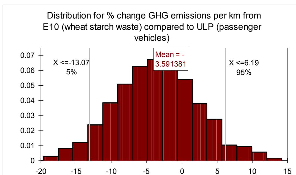
Figure A91. Distribution of percentage change in greenhouse gas emissions from E10 (wheat starch waste) compared to ULP (passenger vehicle)
