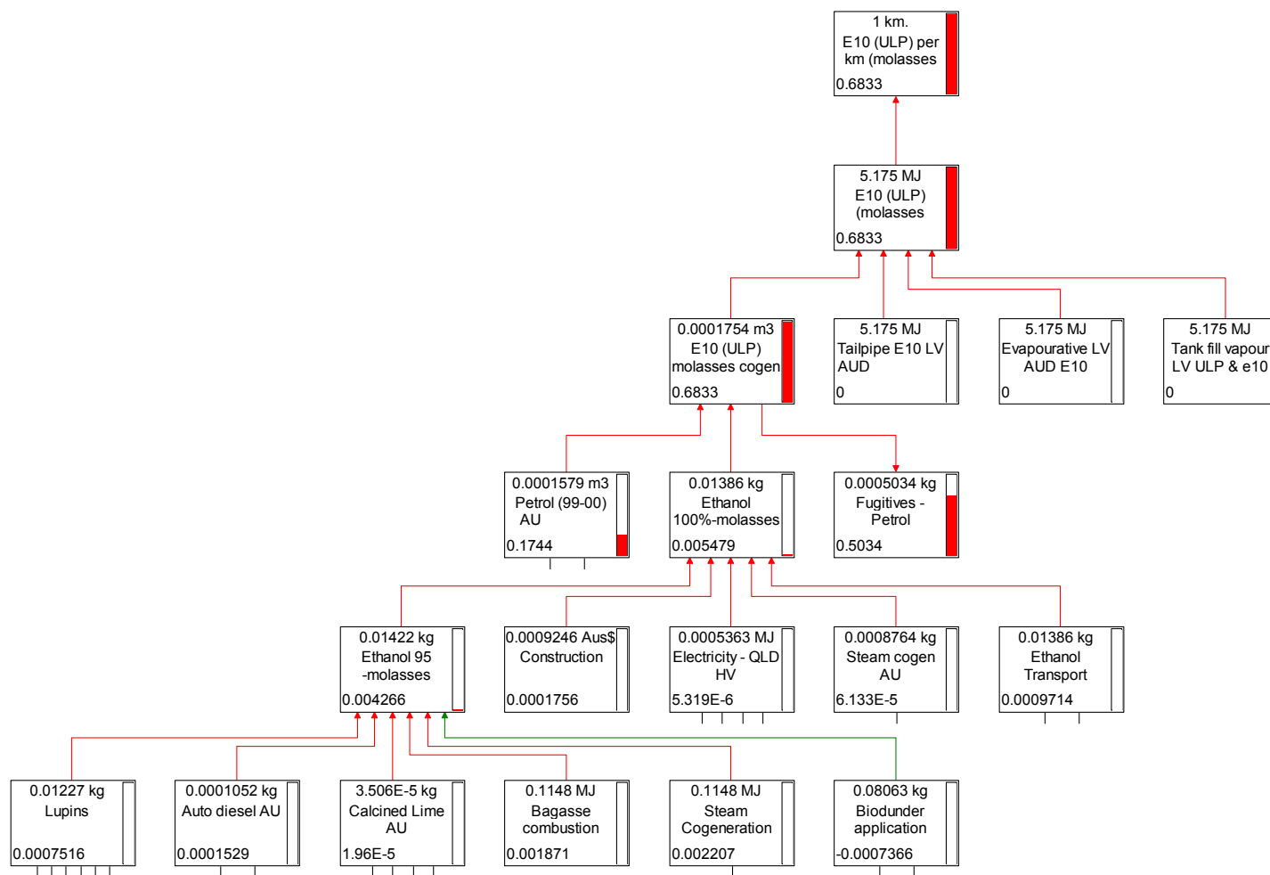
Figure A53. Ethanol (E10 - molasses co-generation) emissions in g NMHC per km (standardised passenger car)
