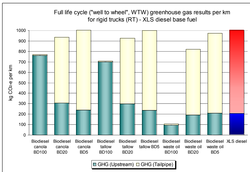
Figure 13. Full life cycle GHG emissions from biodiesel BD100, BD20, and BD5, compared to XLS diesel (rigid truck)
