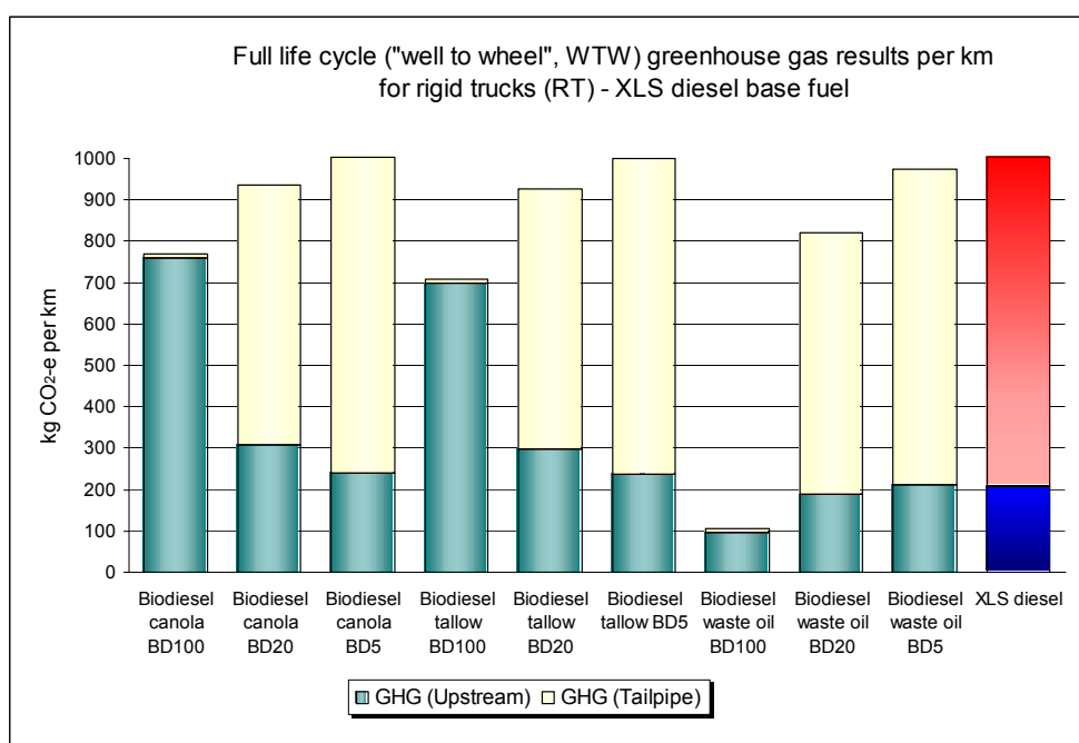
Figure A22. Fuel life cycle GHG emissions from biodiesel BD100, BD20, and BD5, compared to XLS (rigid truck)
