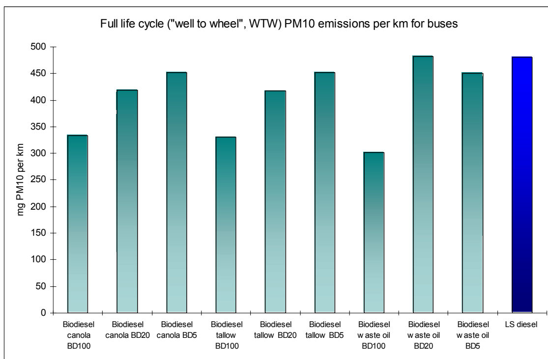
Figure A34. Fuel life cycle PM emissions from biodiesel BD100, BD20, and BD5, compared to LSD (buses)
