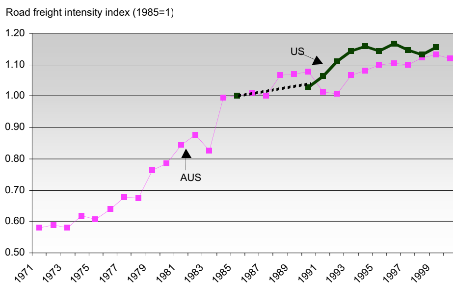
FIGURE 3.2 RATIO OF ROAD FREIGHT TONNE-KILOMETRES TO GDP (1985=1)
