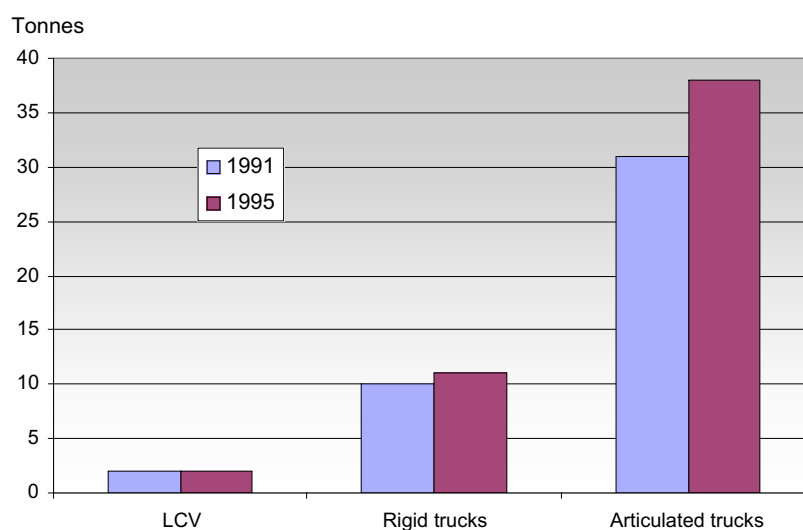
FIGURE 4.2 AVERAGE GROSS VEHICLE/COMBINATION MASS (TONNES, 1991–1995)
